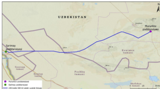
Figure 1. Sarimay-Muruntau OHTL's route
