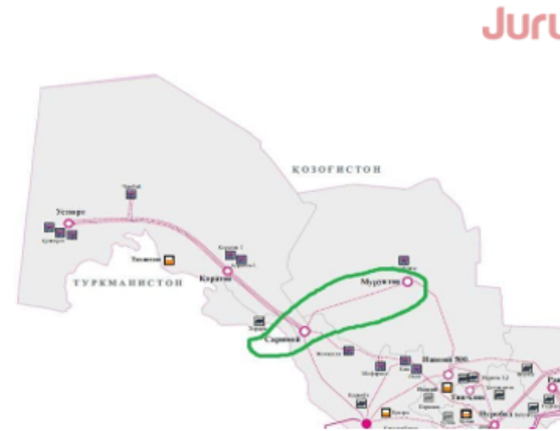
Figure 2. Sarimay-Muruntau OHTL's layout
